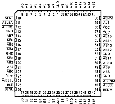
SN74BCT2423 . . . FN PACKAGE (TOP VIEW)
