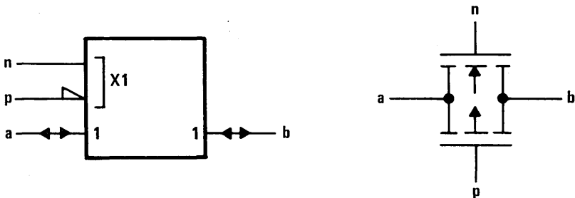
Figure 13. CMOS Transmission Gate Symbol and Schematic
