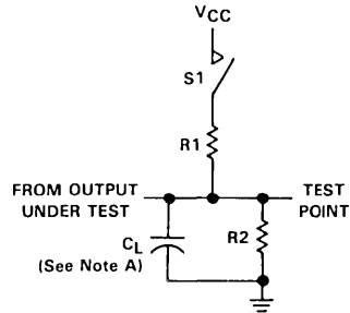
LOAD CIRCUIT FOR NuBus™ INTERFACE
