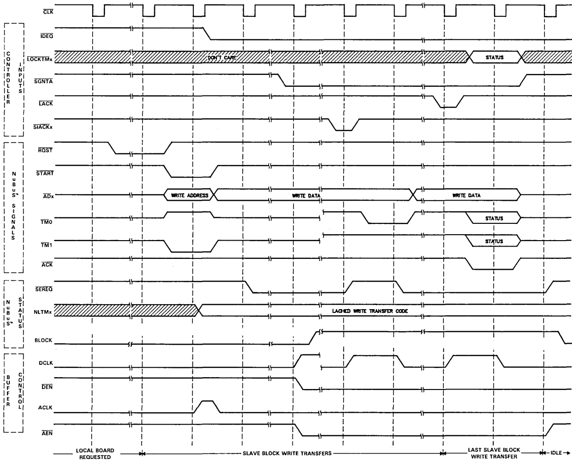
FIGURE 15. SLAVE BLOCK-WRITE TRANSFER CYCLE
