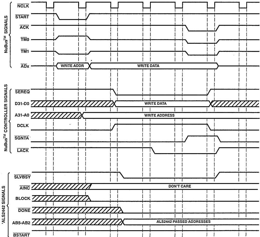
FIGURE 4. TYPICAL NONBLOCK WRITE TRANSFER CYCLE
