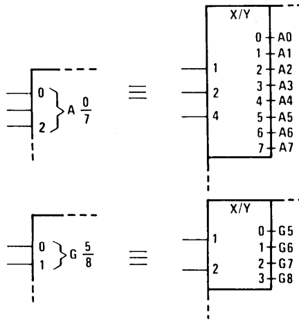
Figure 31. Use of the Binary Grouping Symbol
