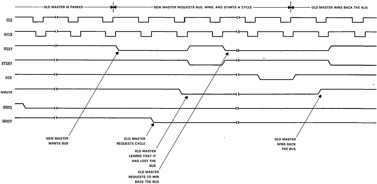
FIGURE 16. NuBus™ CYCLES FROM THE PARKED POSITION
