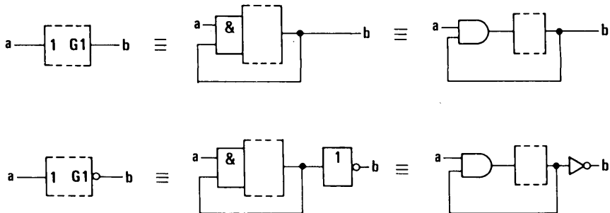
Figure 5. G Dependency Between Outputs and Inputs
