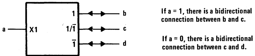
Figure 12. X (Transmission) Dependency
