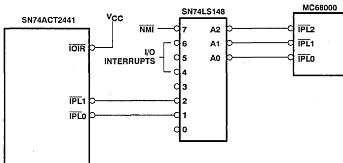
Figure 3. Expanding Interrupts to the MC6800
