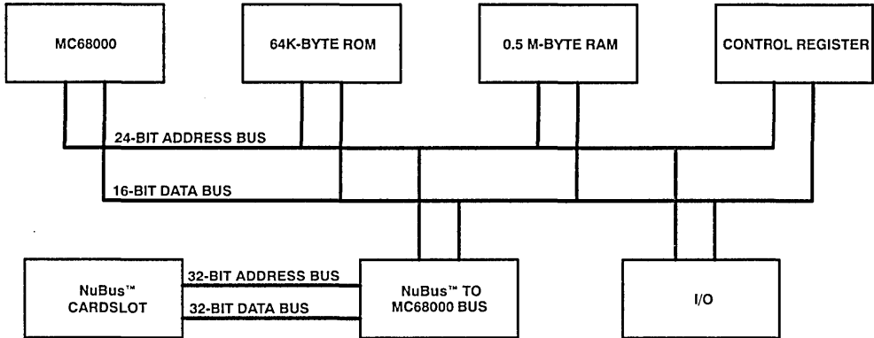
Figure 7. System Block Diagram Showing Data Paths
