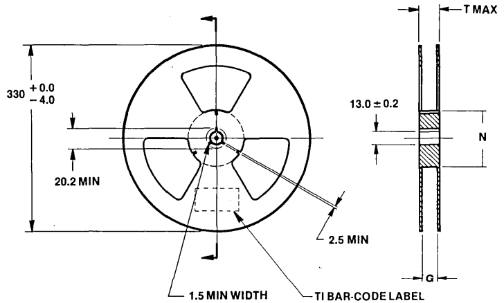
Figure 6 Reel Dimensions
