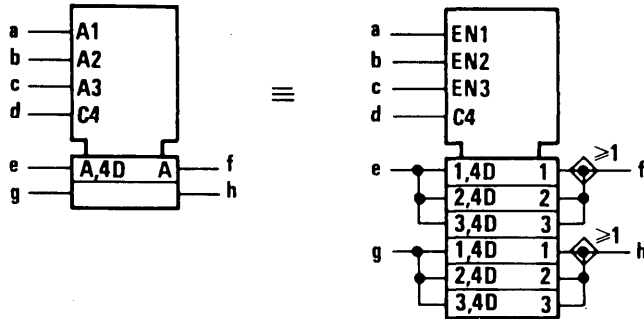
Figure 23. A (Address) Dependency
