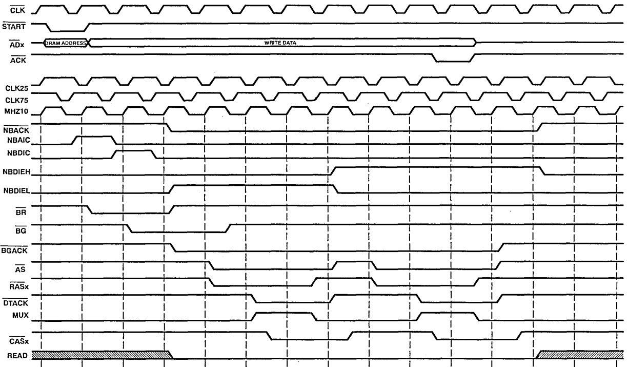
Figure 12. 32-Bit NuBus™ DRAM Write Cycle
