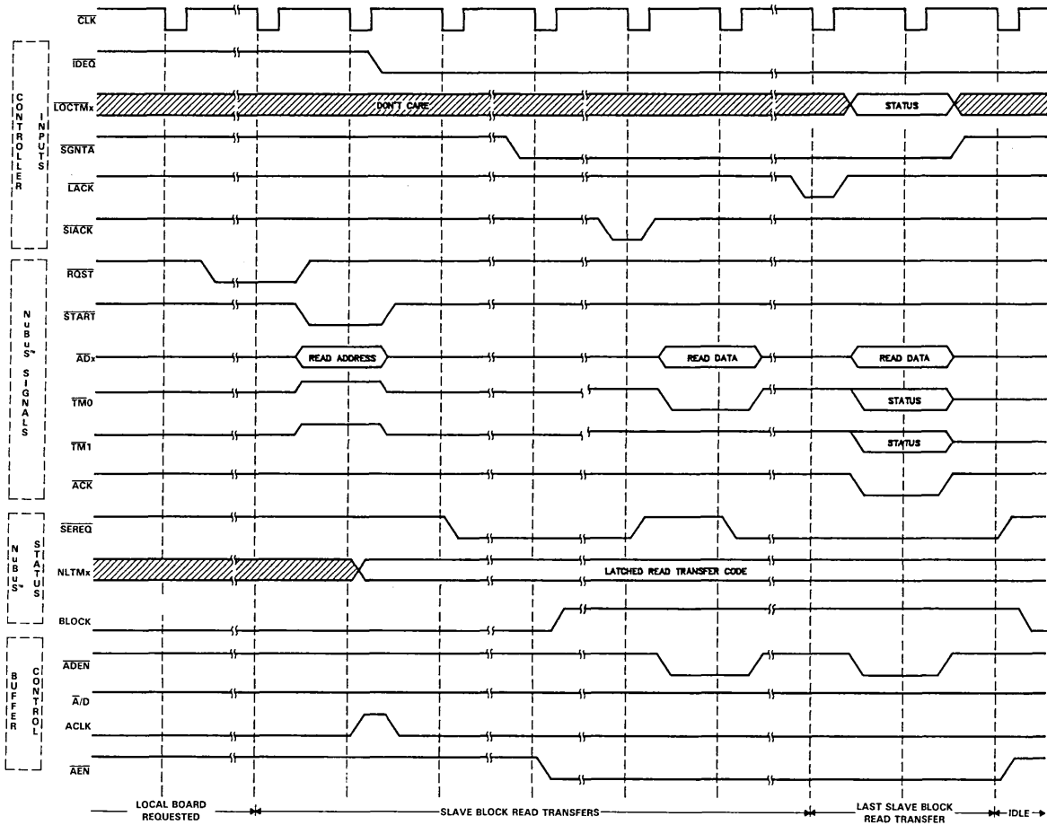
FIGURE 14. SLAVE BLOCK-READ TRANSFER CYCLE
